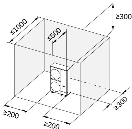
Figure 2-3.3: One outdoor unit installation (unit: mm)
