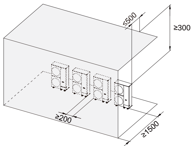
Figure 2-3.8: More than one outdoor unit installation (unit: mm)
