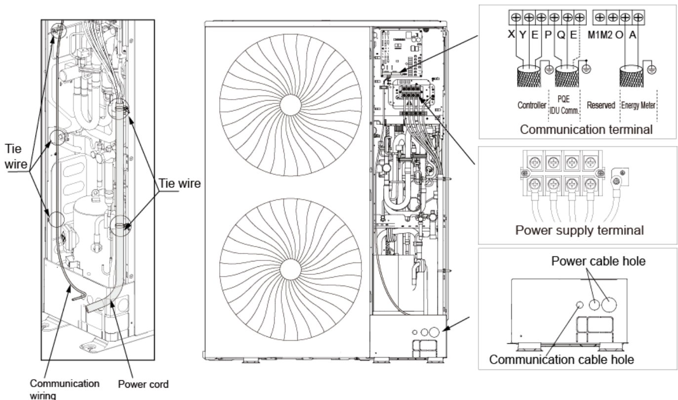
Figure 3-9.1: Wiring layout
