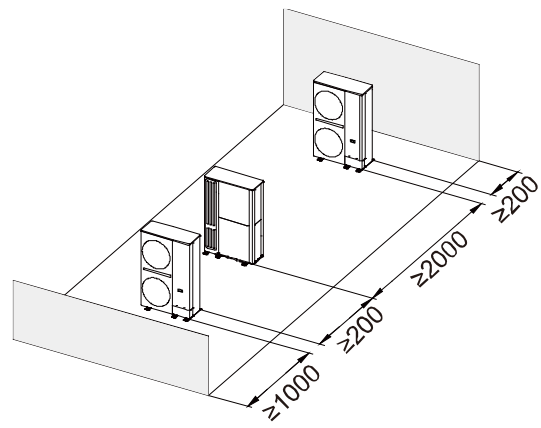
Figure 2-3.17: One outdoor unit installation (unit: mm)
