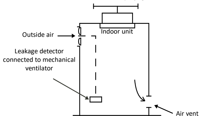
Figure 3-4.5: Mechanical ventilator controlled by refrigerant leak detector
