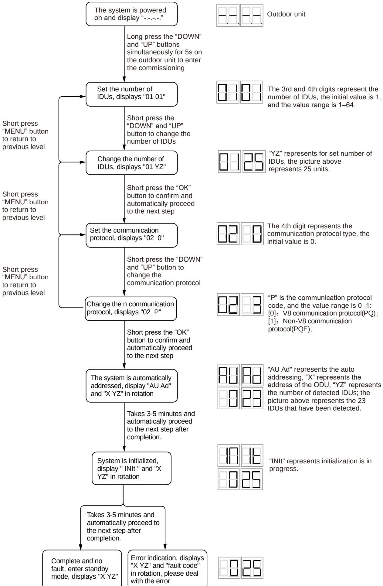
Figure 3-11.1: Test Run Procedure
