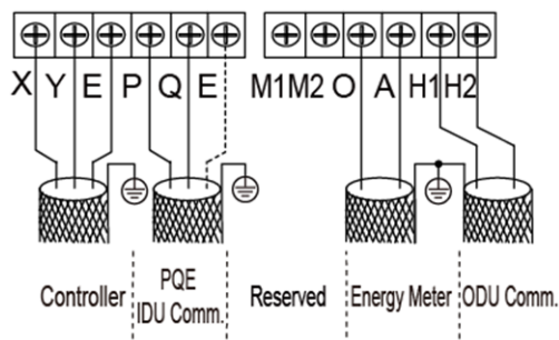
Figure 3-9.11: Outdoor unit communication terminals
