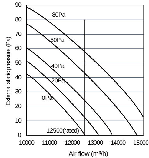
Figure 3-3.5: 14HP units fan performance
