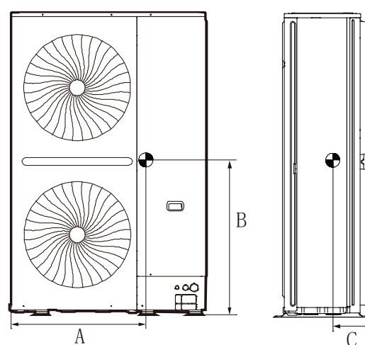
Figure 3-2.5: 8-22HP Center of gravity
