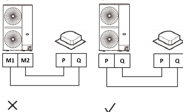
Figure 3-9.5: Communication wiring
