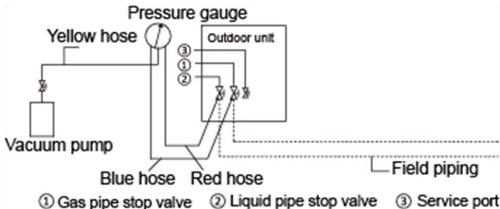
Figure 3-5.15: Vacuum drying
