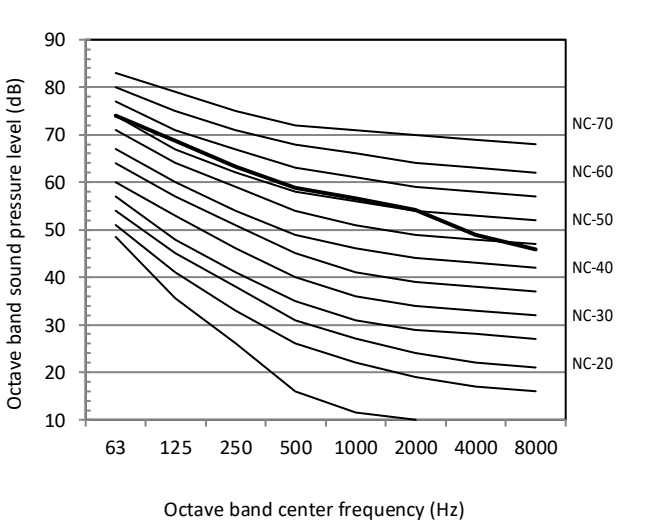
Figure 2-10.6: 16HP octave band level
