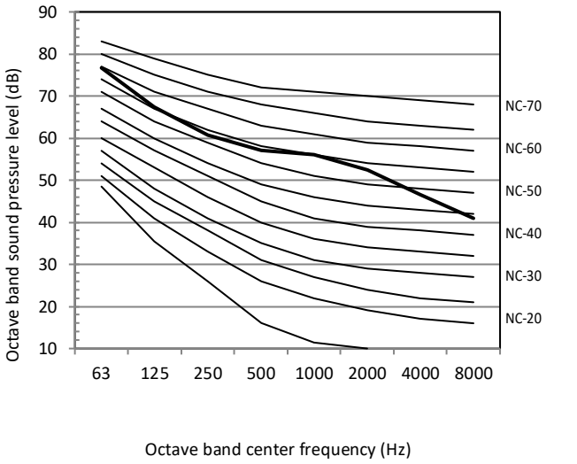
Figure 2-10.4: 12HP octave band level
