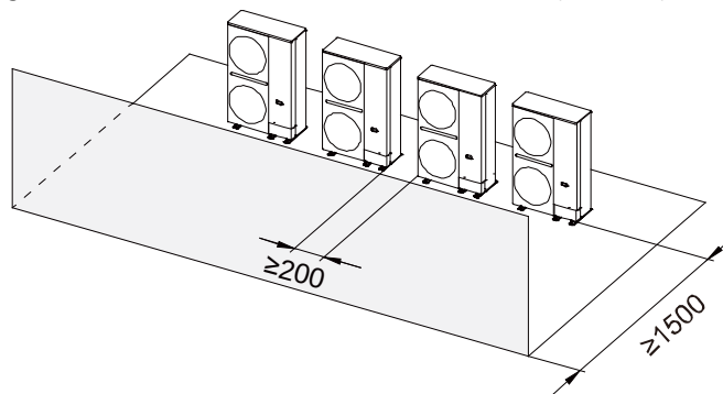
Figure 2-3.6: More than one outdoor unit installation (unit: mm)
